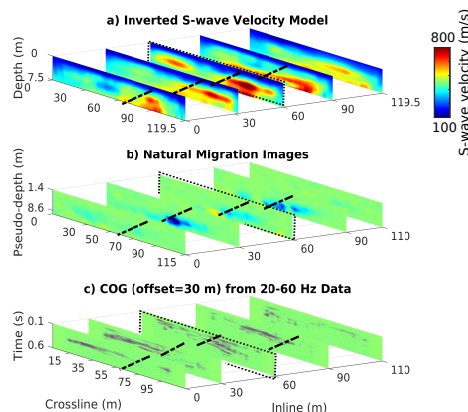
Figure 8: Slices of a) the inverted S-wave velocity model, b) natural migration images (Liu et al., 2017) and c) common offset gathers (offset is 30 m). The dashed lines indicate the location of the interpreted Qadema fault.
