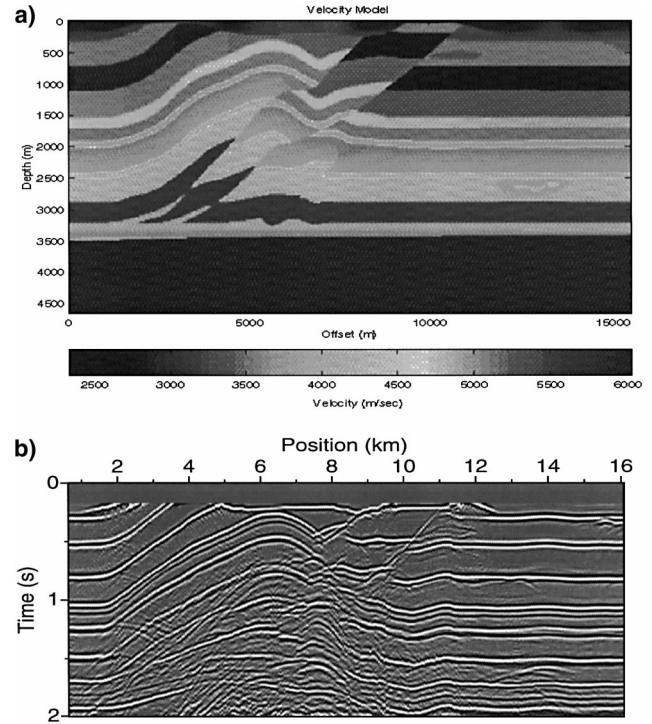
FIG. 7. Test with the Overthrust velocity model. (a) Overthrust velocity model associated with the Phase A data set (SEG/EAGE 3-D Modeling Series No. 1), (b) zero-offset Phase A data set associated with the SEG Overthrust model.
