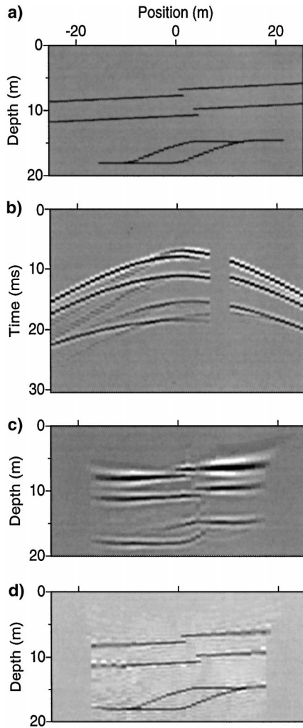
FIG. 6. The fault model used to demonstrate the capability of LSM to image hidden or weaker diffractors. (a) The fault model, (b) synthetic seismograms, (c) Kirchhoff migrated section, (d) least-squares migrated section.
