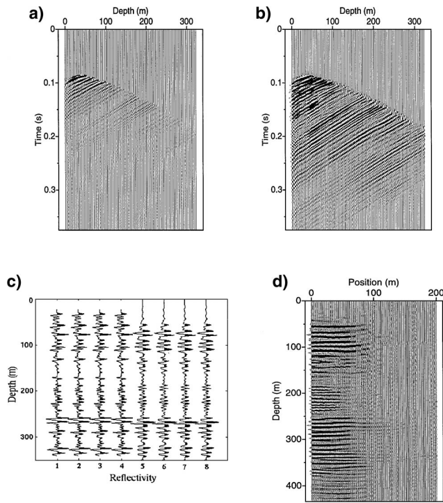
FIG. 14. The Friendswood RVSP experiment. (a) Common-receiver gather predicted with Kirchhoff migrated section, (b) common-receiver gather predicted with least-squares migrated section, (c) well-log synthetics (traces 1–4) and migrated data trace (5–8) at the source well, (d) the stacked migrated section after residual moveout correction.
