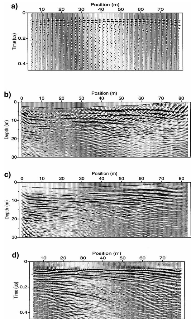
FIG. 11. Test with the 1:4 spatially subsampled 8-m common-offset section of profile A. (a) Observed radargrams, (b) Kirchhoff migrated section, (c) least-squares migrated section, (d) predicted radargrams using the least-squares migrated section.
