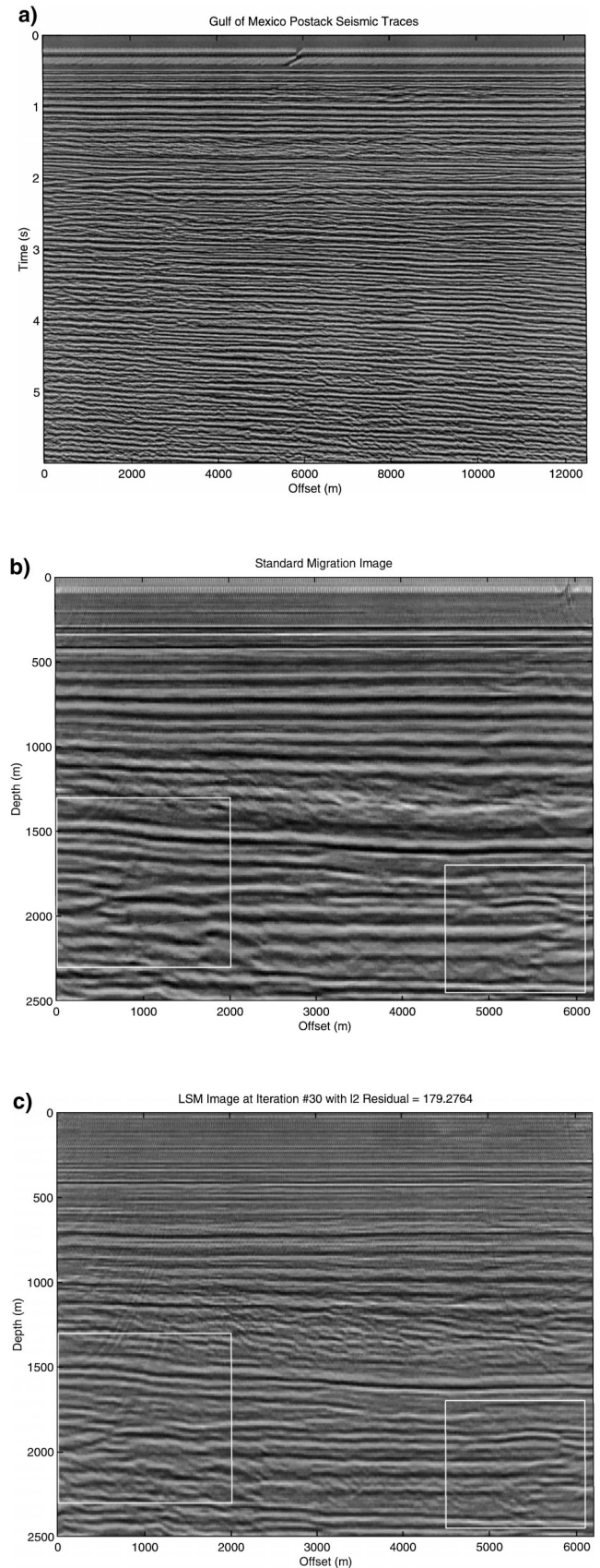
FIG. 15. The Gulf of Mexico data experiment. (a) Poststack traces; (b) Poststack Kirchhoff migrated section; (c) Poststack LSM migrated section. It appears that the LSM migrated section is more highly resolved than the Kirchhoff migration section.
