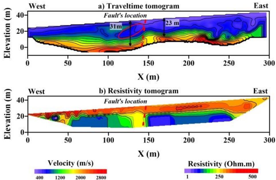
Figure 5: a) The seismic travel-time tomogram and b) the resistivity tomogram. The red-dashed line shows the suggested location of the fault, extrapolated from the fault's location at the surface. The red-solid ellipse shows a low-velocity region within the tomogram, which might be interpreted as a colluvial wedge associated with the fault.
