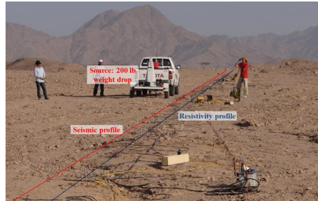
Figure 3: A photo taken during the data acquisition. Both the seismic (red line) and the resistivity (blue line) profiles are shown here. The photo is taken along the profile towards the east.
