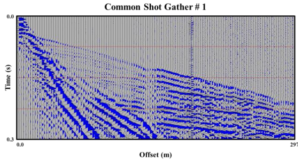
Figure 4: An example common shot gather, showing a high signal-to-noise ratio, with first arrivals that can easily be picked.
