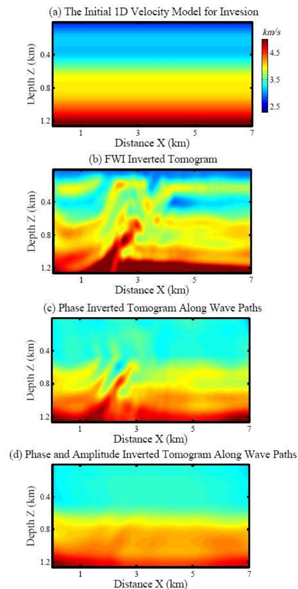
Figures 4: (a) The 1D initial velocity model, the tomograms inverted by (b) conventional FWI, by (c) only phase along
