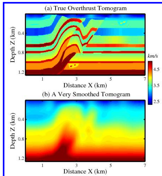
Figure 3: The (a) true and the (b) smoothed Overthrust velocity models.
