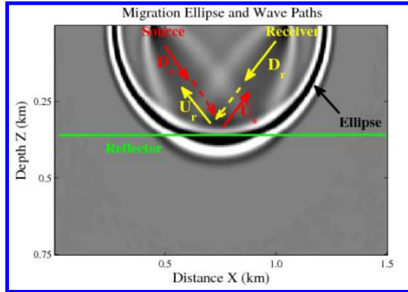
Figure 1: The migration ellipse and wave paths.
