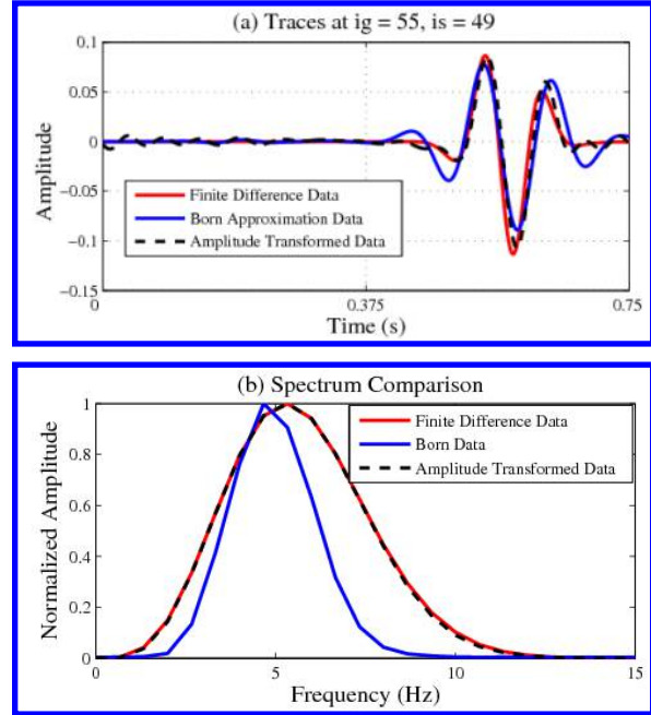
Figure 2: (a) The reflection data calculated by finite difference scheme, the demigration data calculated by Born modeling, and the transformed demigration data using equation 7; (b) their spectrum. The data for comparison are calculated based on a two layered velocity model.
