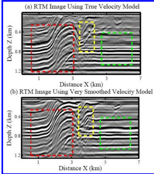
Figure 5: RTM images using (a) the true overthrust velocity model, and (b) its very smoothed version.
