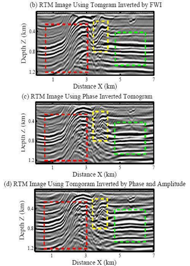
Figure 6: RTM images using (a) the 1D initial velocity model, the tomograms inverted by (b) conventional FWI, by (c) only phase along reflection wave paths, and by (d) both amplitude and phase along reflection wave paths.
