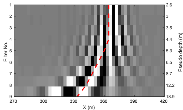
Figure 4: The normalized stacked migration images at z = 0 and x from 270 m to 420 m, and computed from the synthetic data with different narrow-band filters. The right y axis is pseudo depth calculated from 1/3 the wavelength, and the red dashed line is the interpreted fault position corresponding to the red dash line in Figure 2.
